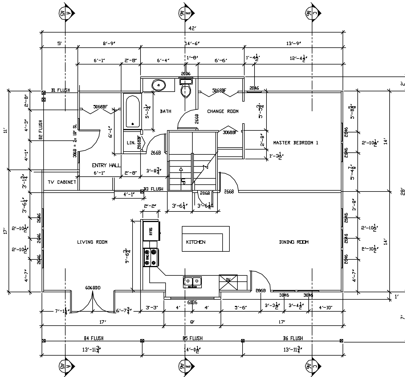
MAIN FLOOR PLAN 1150 SF
