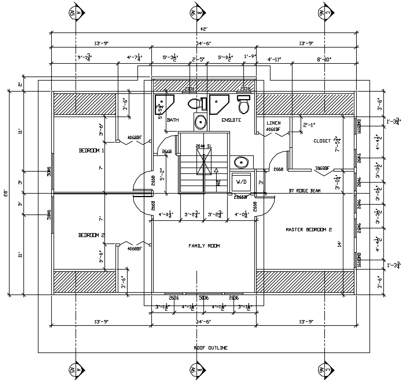
UPPER FLOOR PLAN 1205 SF
